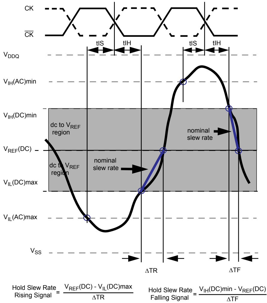
Figure 17. Illustration of nominal slew rate for t IH
