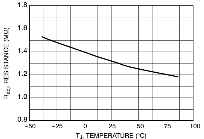
Figure 4. ADJ Pin Resistance vs. Temperature
