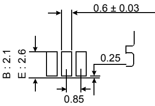
Detail B,E
