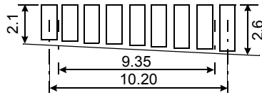
Detail C
