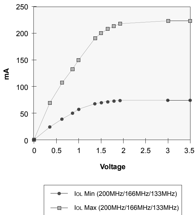
Figure 5. 200MHz/166MHz/133MHz Pull-down
