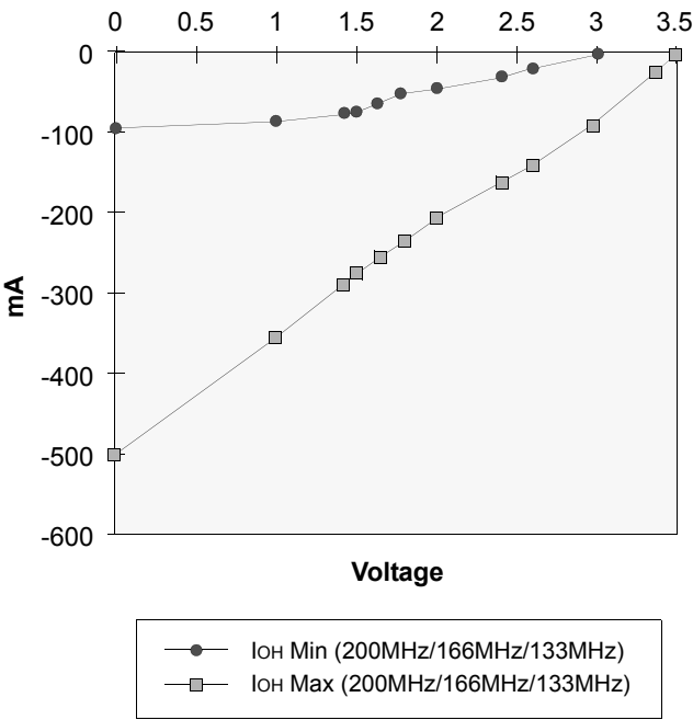
Figure 4. 200MHz/166MHz/133MHz Pull-up
