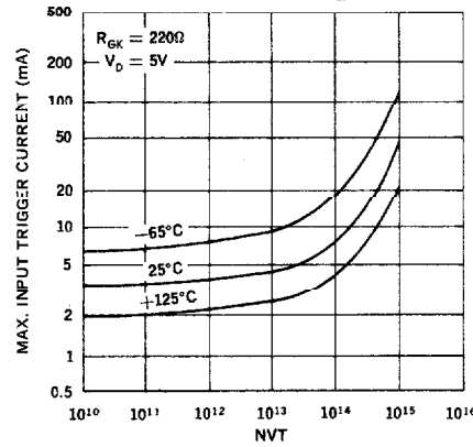
6. Max. Input Trigger Current vs. Neutron Dosage
