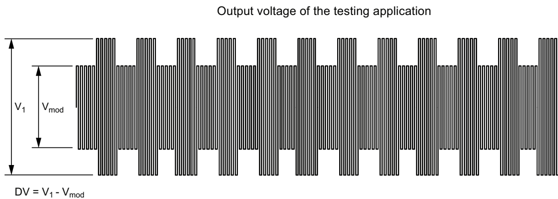
Figure 6-3. Measurement of the Modulation Range DV
