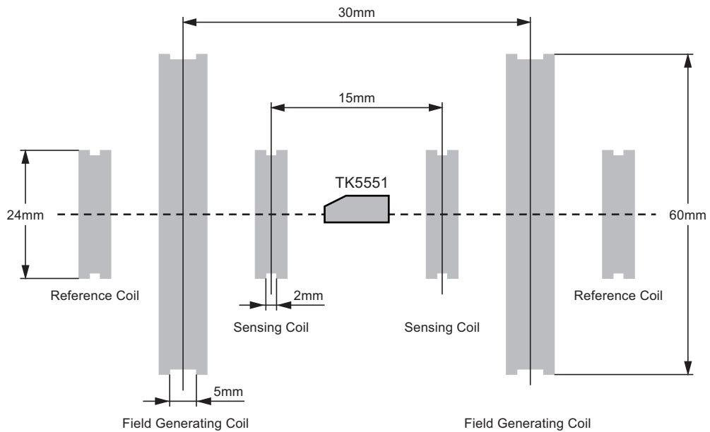
Figure 7-2. Testing Geometry
