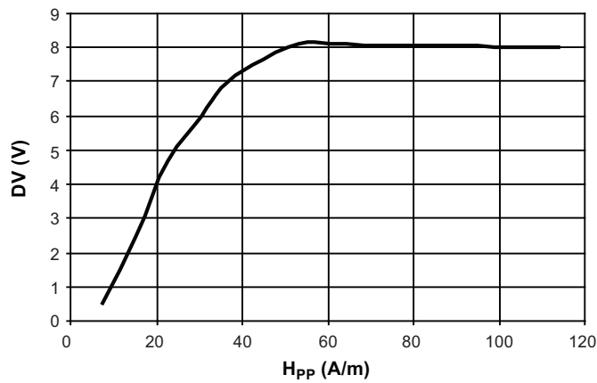
Figure 6-3. Measurement of the Modulation Range DV
