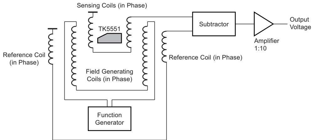
Figure 7-1. Testing Application
