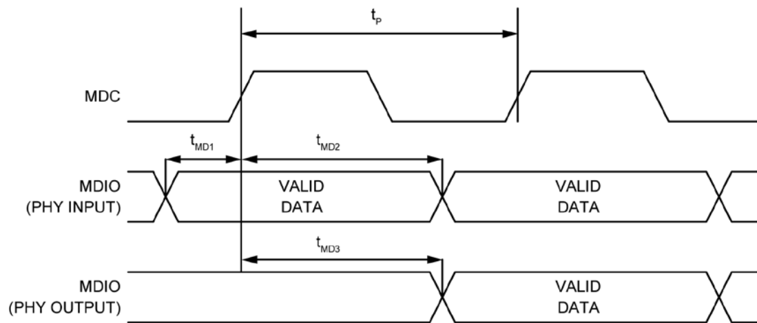
Figure 13. MDC/MDIO Timing
