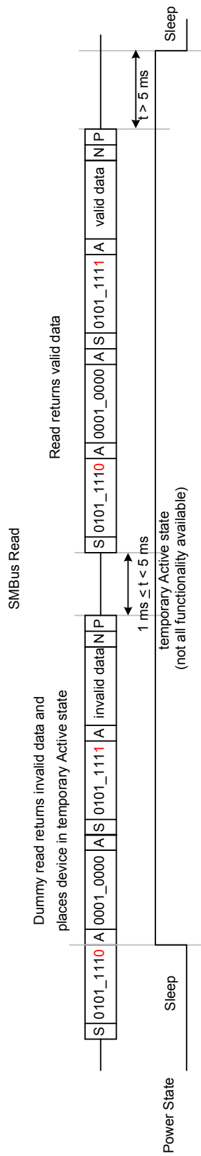
Figure 2.6 Wake Via SMBus Read with S0 = '0'
