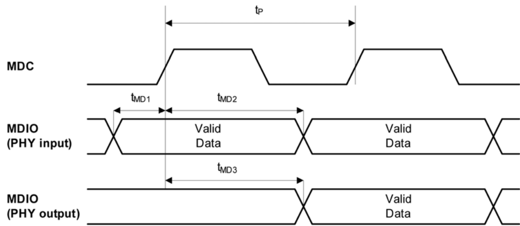
Figure 17. MDC/MDIO Timing
