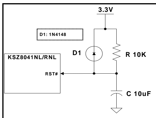
Figure 19. Recommended Reset Circuit
