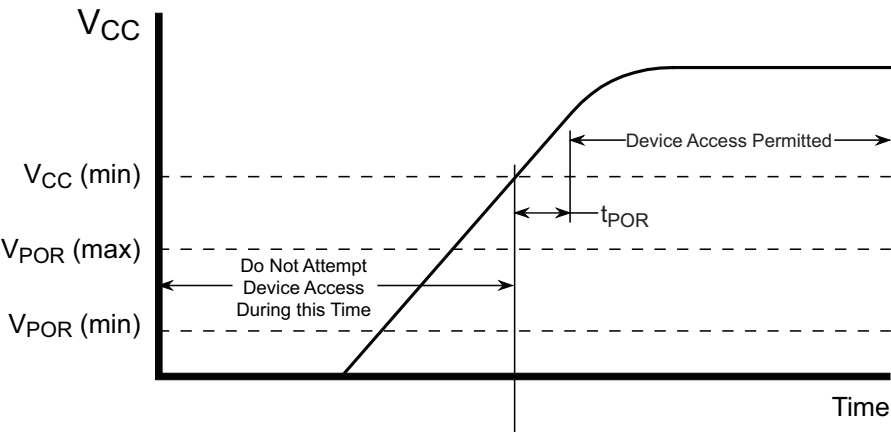
Figure 8-2. Power-Up Timing
