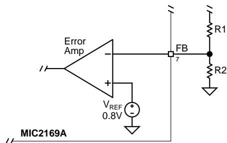
Figure 2. Voltage-Divider Configuration
