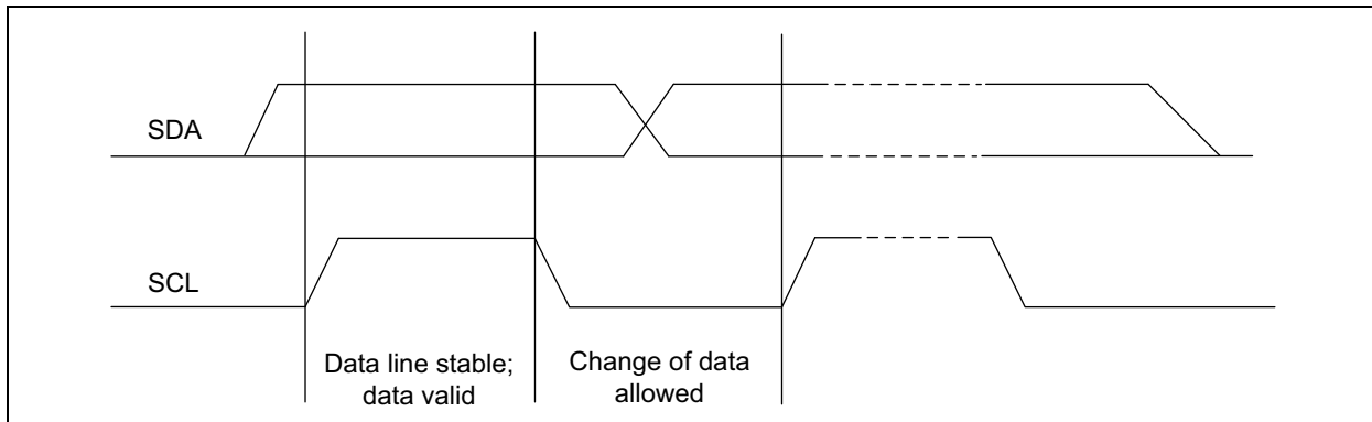
FIGURE 6-1: Bit Transfer.
