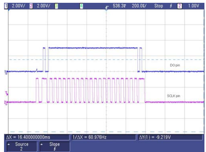
Figure 16. All Bits D19 through D0 = 1
