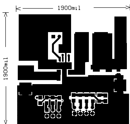
Figure 5c. Top Layer
