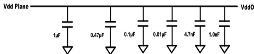
Figure 3. Recommended decoupling for each VDDO
