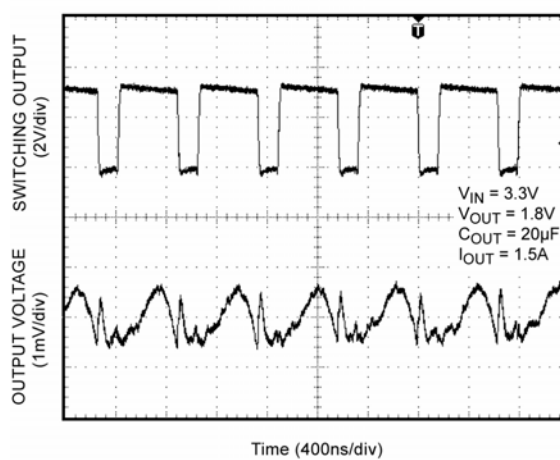
Output Ripple
