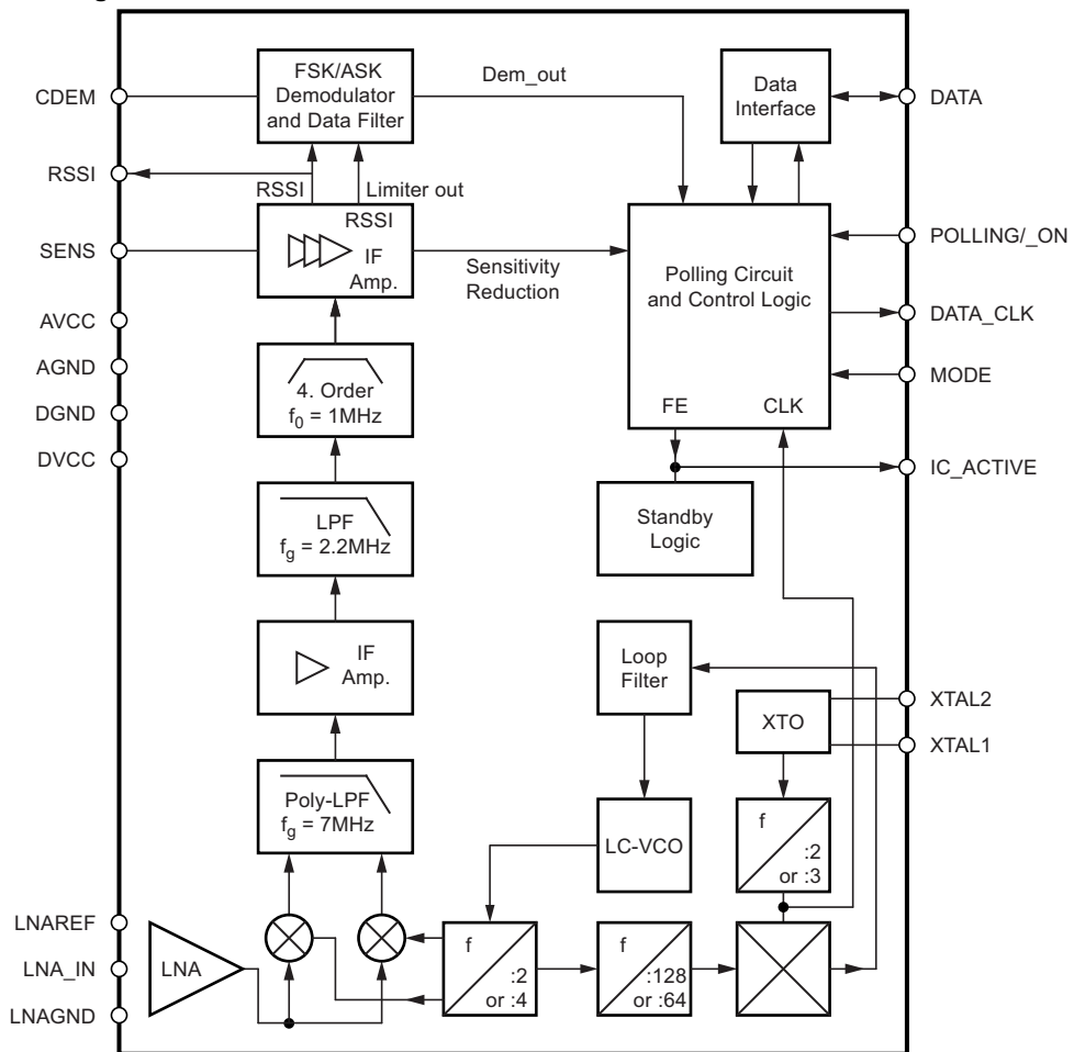
Figure 1-2. Block Diagram
