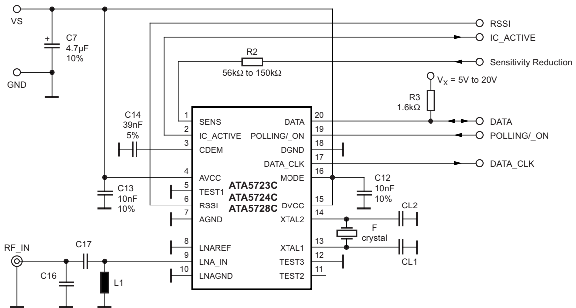
Figure 14-1. Application Circuit: f_{RF} = 315MHz^{(1)} , 433.92MHz or without SAW Filter
