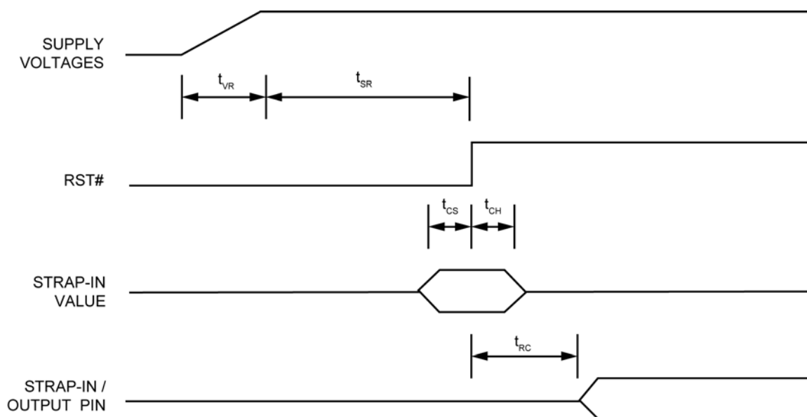
Figure 18. Power-Up/Reset Timing
