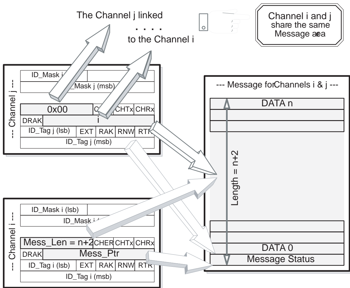
Figure 31. Linkage Mechanism
