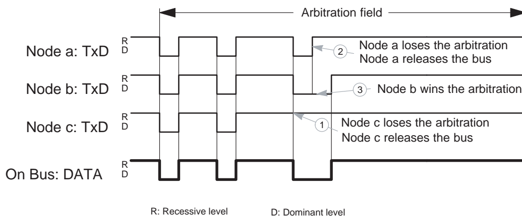
Figure 5. CSMA/CD Arbitration
