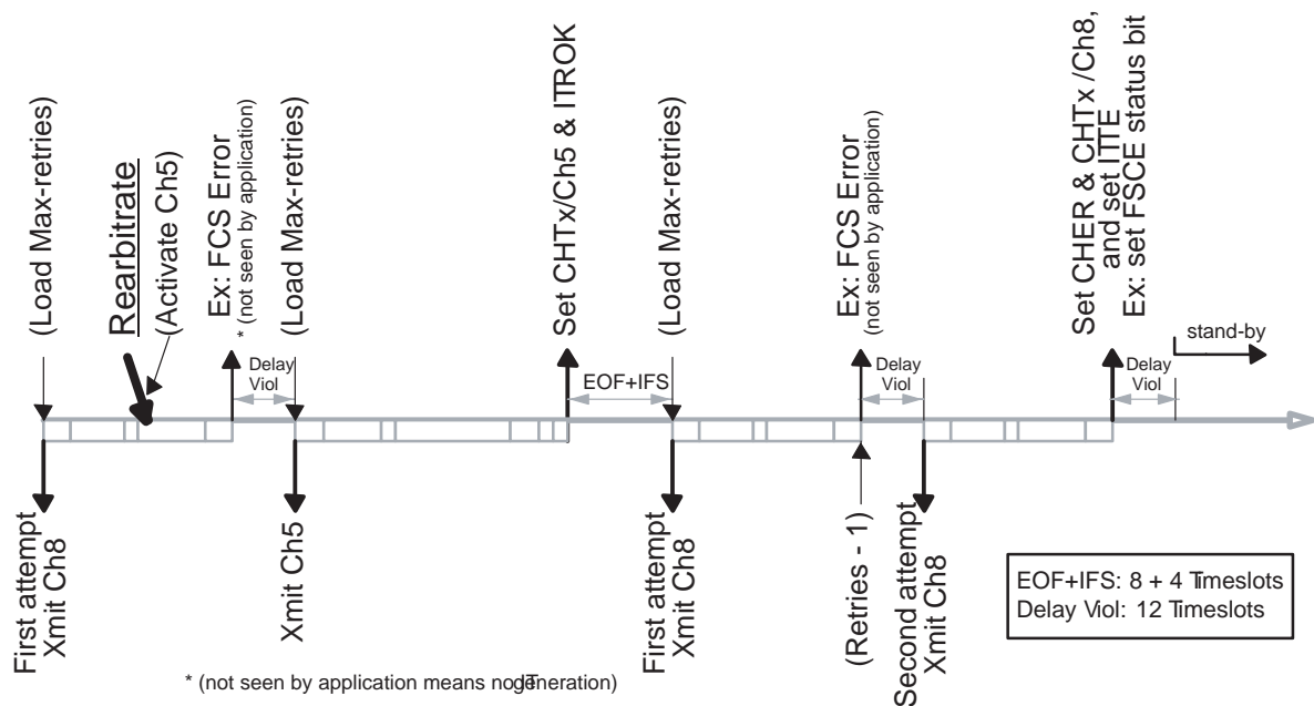
Figure 26. Rearbitrate Example
