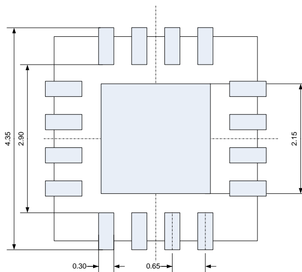
Figure 5: Package Drawing
