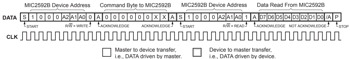
Figure 11. READ_BYTE Protocol
