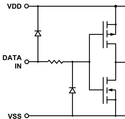
Logic Inputs
