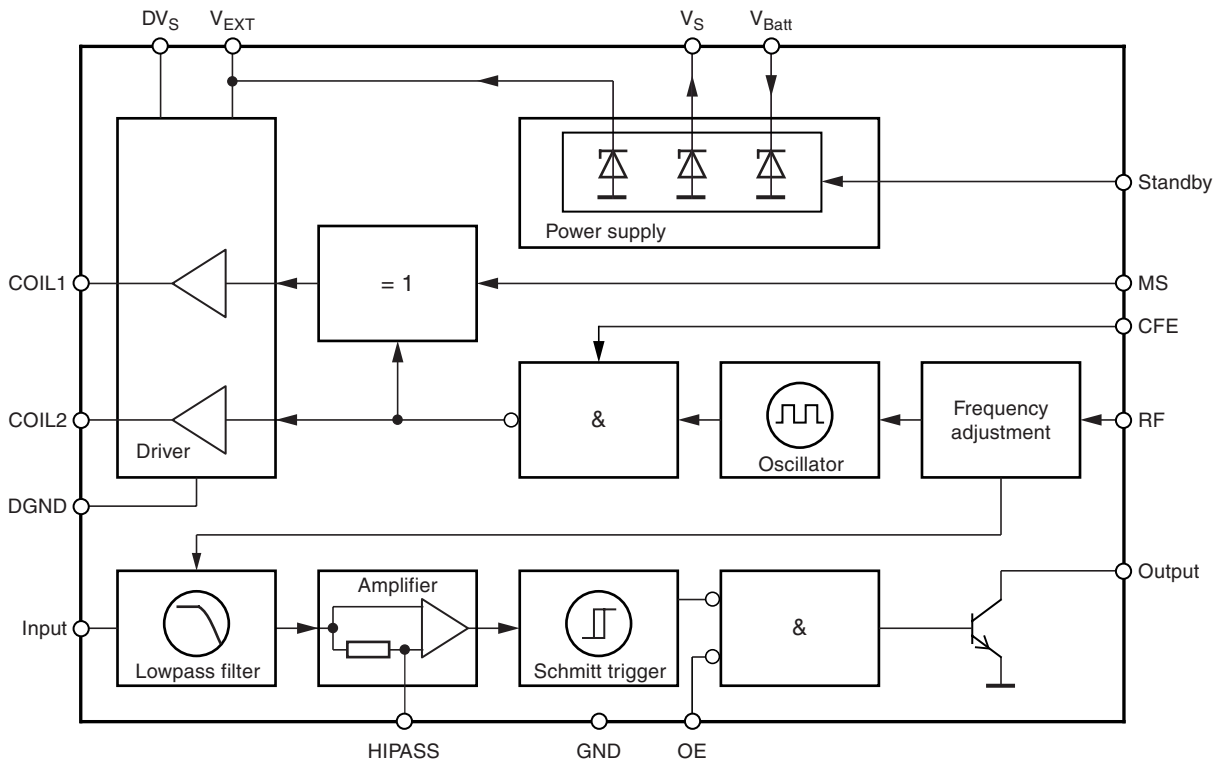
Figure 1-2. Block Diagram
