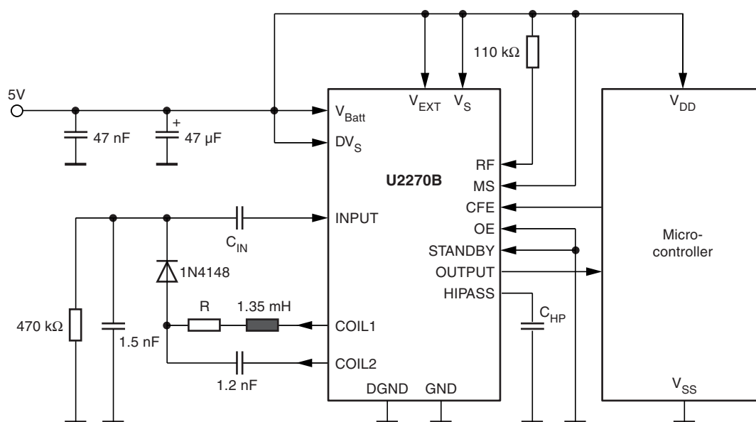
Figure 4-1. Application Circuit 1
