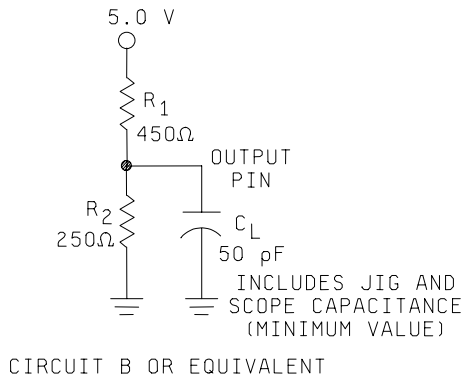
FIGURE 3. Output test circuit.
