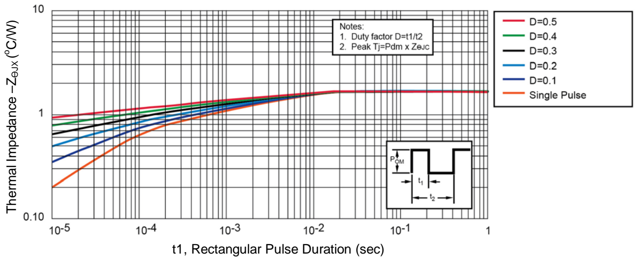
FIGURE 2 Thermal Impedance (for each leg)
