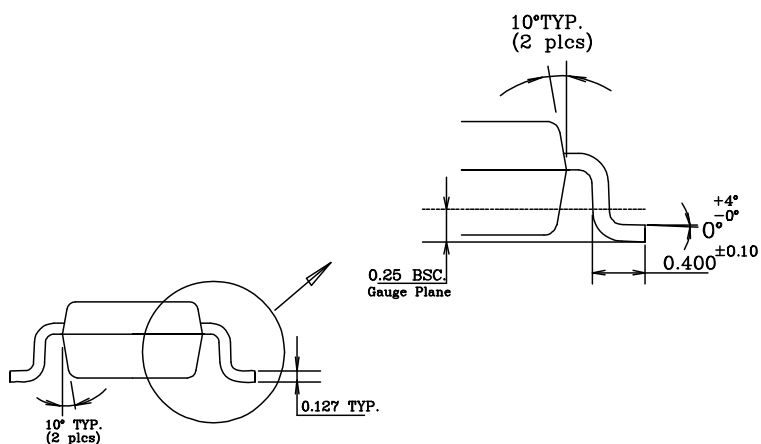
6-Pin TSOT23 (D6)
