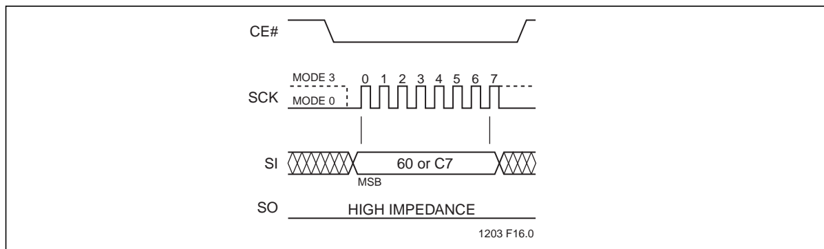
Figure 17: Chip-Erase Sequence
