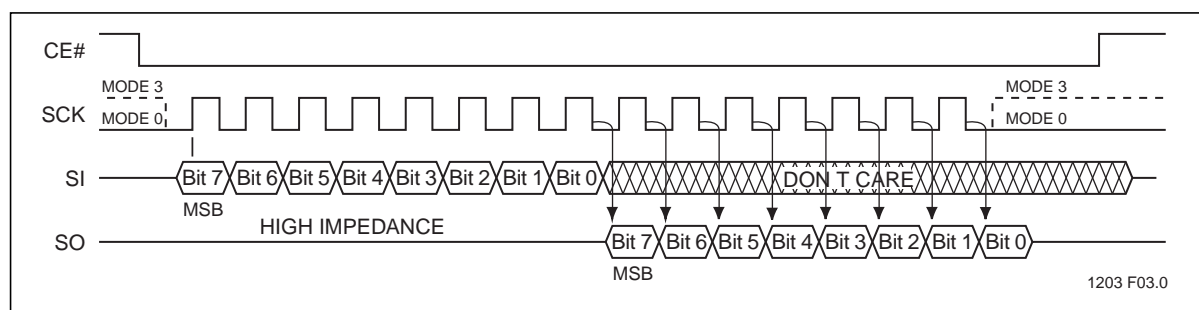
Figure 4: SPI Protocol
