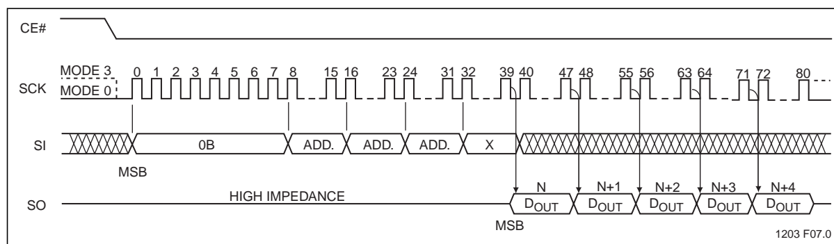
Figure 8: High-Speed-Read Sequence
