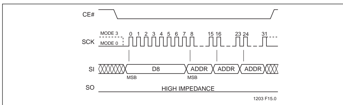
Figure 16: 64-KByte Block-Erase Sequence
