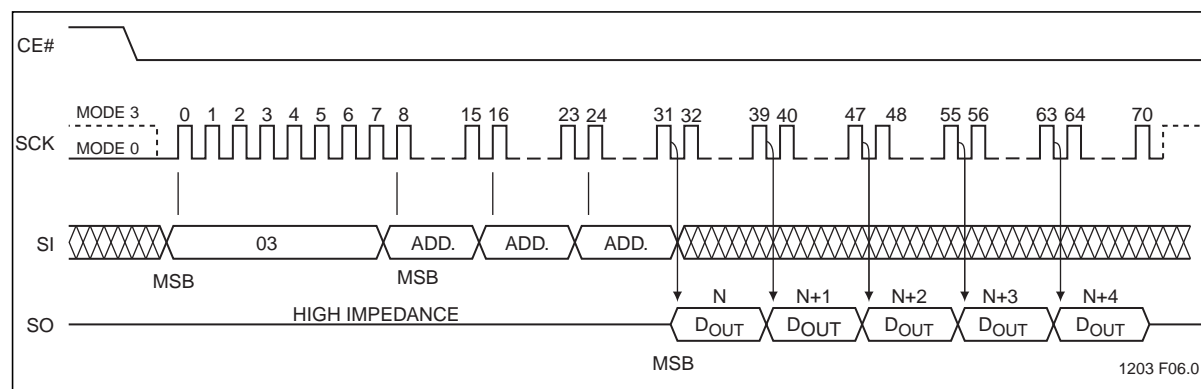
Figure 7: Read Sequence
