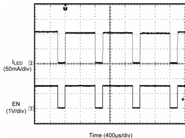
Figure 9. PWM Signal at 80% Duty Cycle ( I_{avg} = 80mA )
