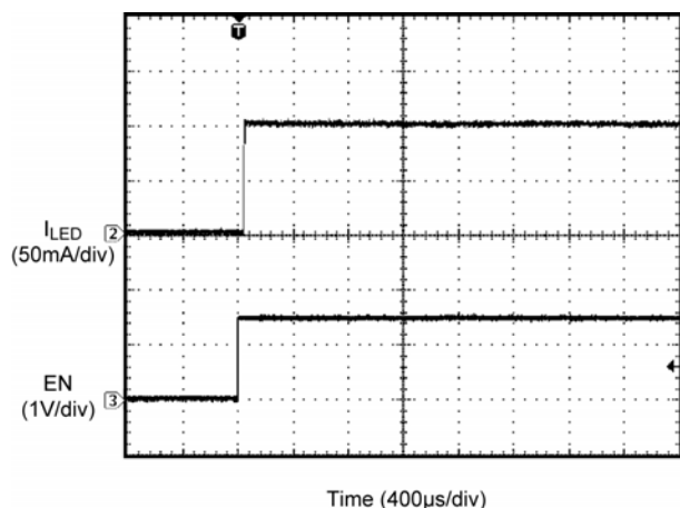
Figure 10. PWM Signal at 100% Duty Cycle ( I_{avg} = 100mA )
