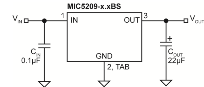
Figure 5. Slot-1 Power Supply
