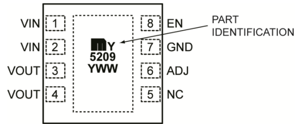
MIC5209YML 8-Pin 3mm x 3mm DFN Adjustable Voltages
