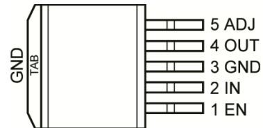
MIC5209BU TO-263-5 Adjustable Voltages
