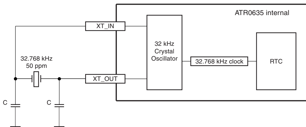
Figure 5-3. Crystal Connection
