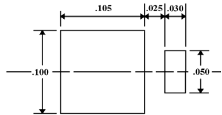
MOUNTING PAD
