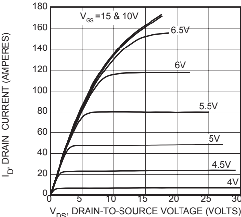
FIGURE 2, LOW VOLTAGE OUTPUT CHARACTERISTICS
