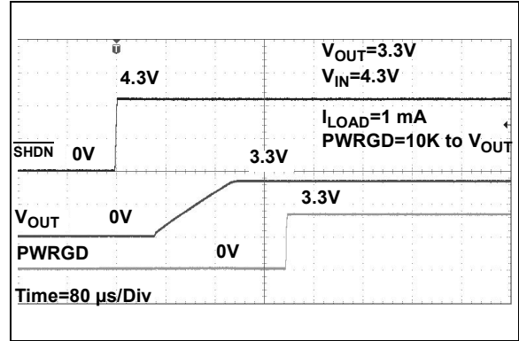
FIGURE 2-28: Start-up from \overline{SHDN} .
