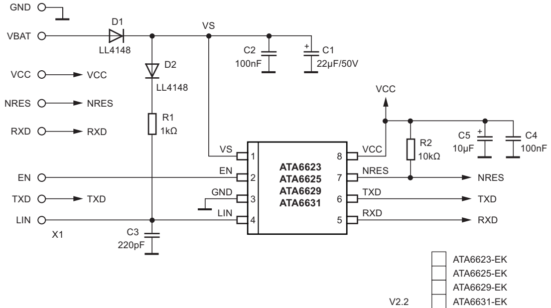
Figure 2-1. Schematic of the Development Board for the Atmel ATA6629/ATA6631
