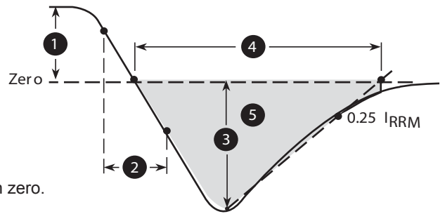
Figure 31. Diode Reverse Recovery Waveform Definition
