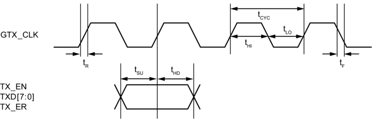
Figure 13. GMII Transmit Timing – Data Input to PHY
