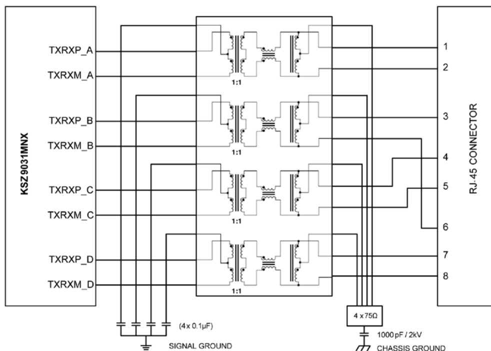
Figure 25. Typical Gigabit Magnetic Interface Circuit
