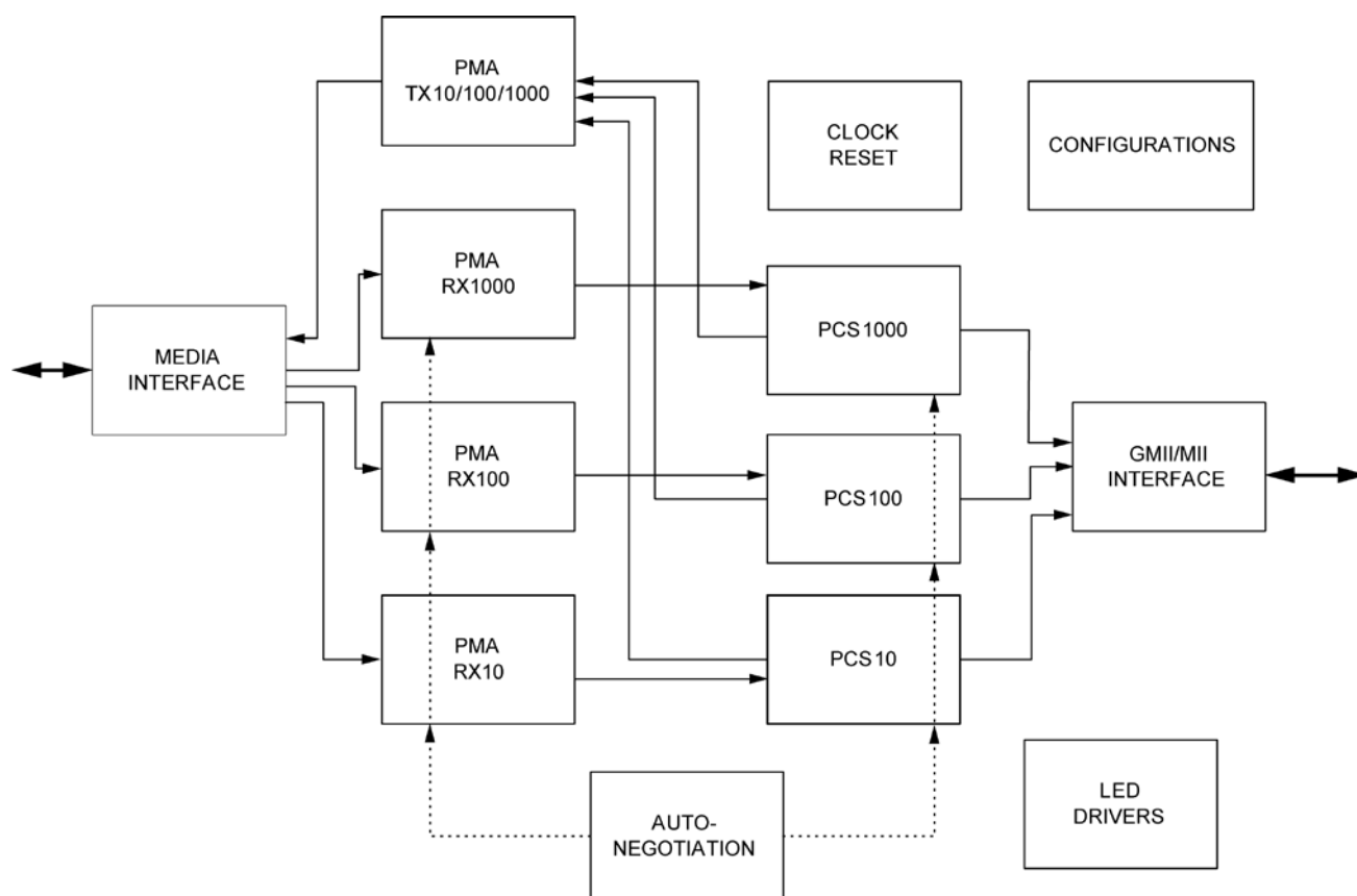
Figure 1. KSZ9031MNX Block Diagram
