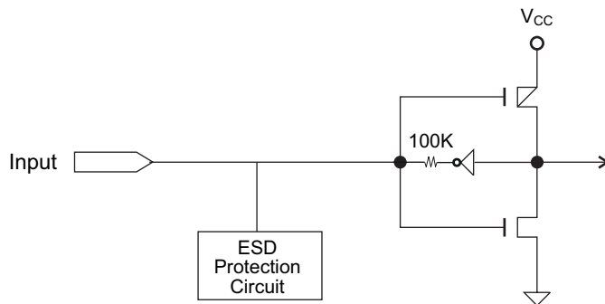
Figure 6-1. Input Diagram
