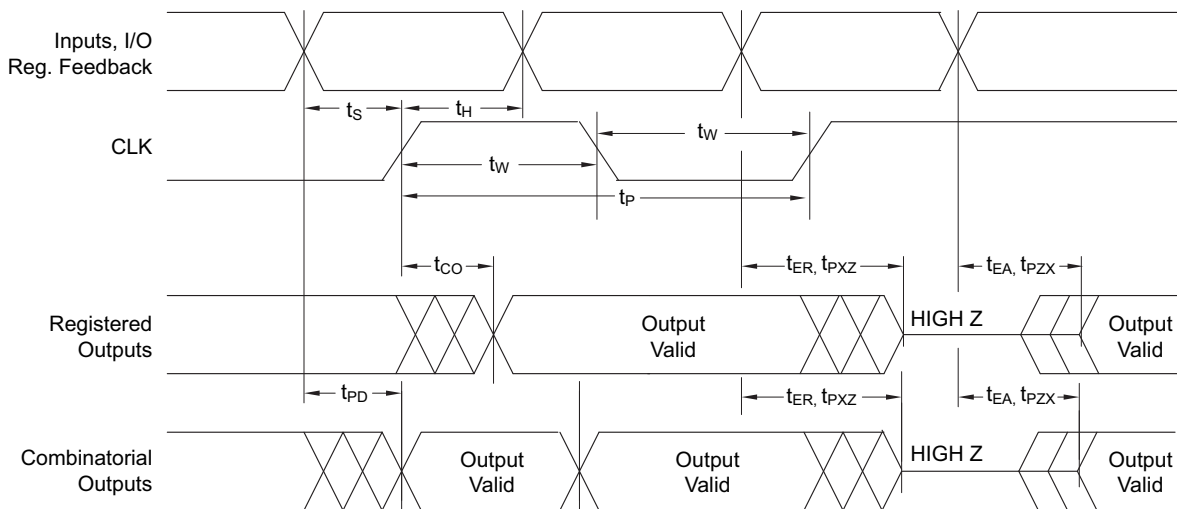
Figure 3-2. AC Waveforms
