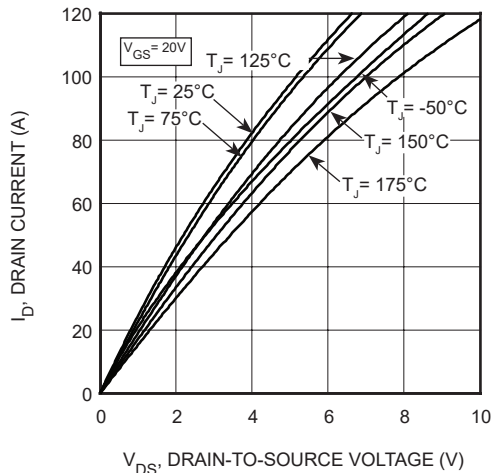
Figure 1, Output Characteristics
