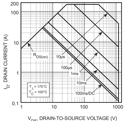
Figure 14, Forward Safe Operating Area
