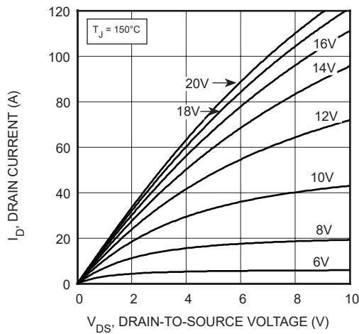
Figure 3, Output Characteristics
