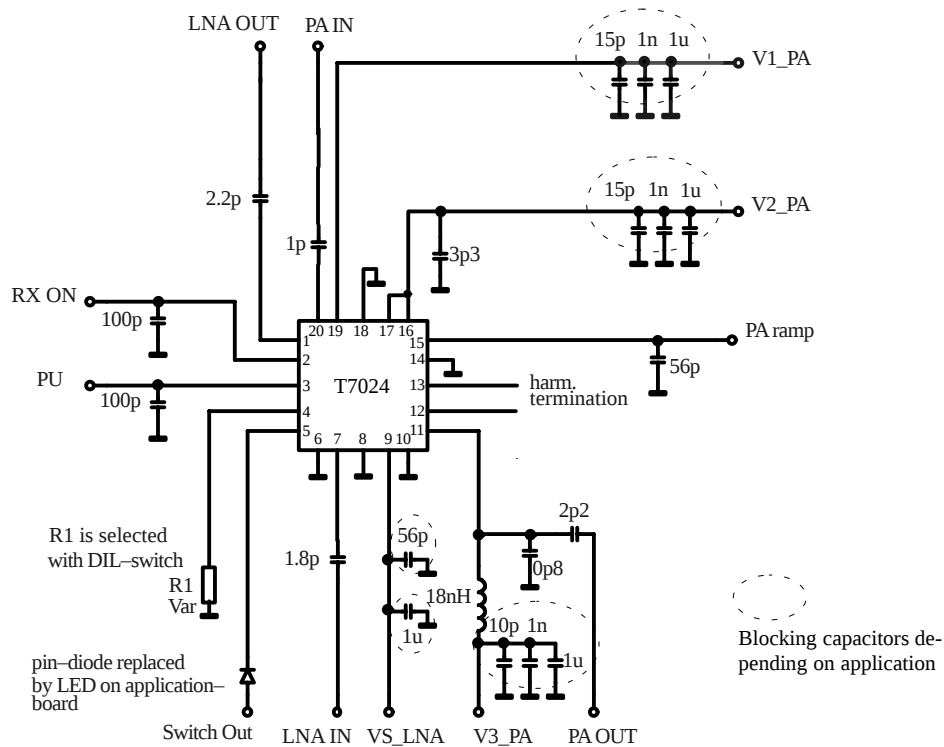
Figure 29. Application board N20
