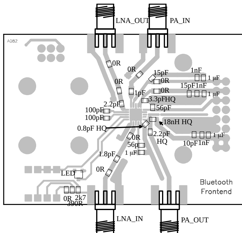
Figure 30. Layout for N20
