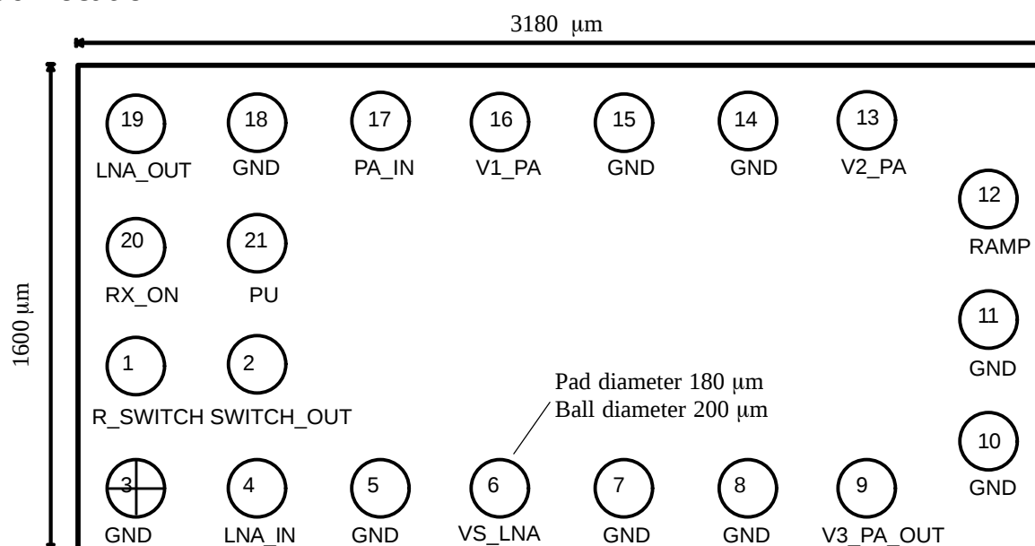
Figure 4. Pad location, die thickness: 450 \mu m
