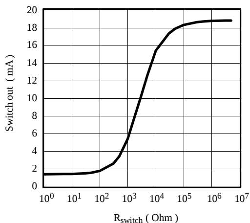
Figure 13. LNA: Typical switch-out current vs. R_{\text{switch}}
