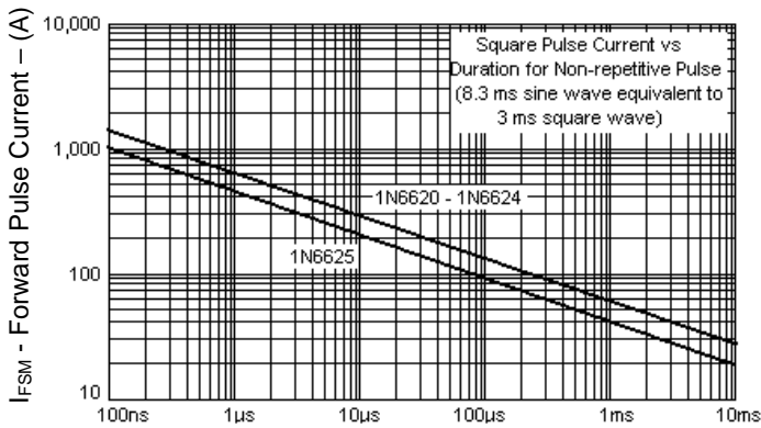
Pulse Duration FIGURE 7 Forward Pulse Current vs. Pulse Duration
