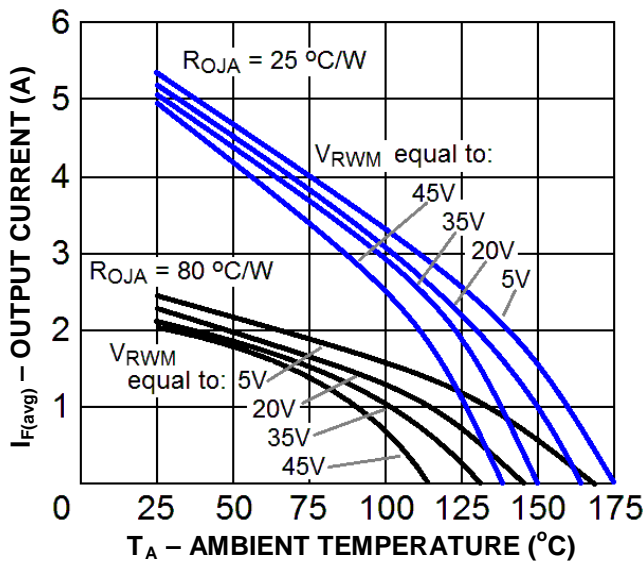
FIGURE 4 – Output Current vs. Ambient Temperature 50% Duty Cycle Application ( I_{F(avg)} and V_{RWM} )
