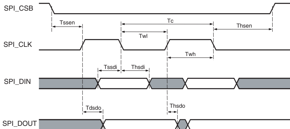
Figure 8-2. SPI Timing
