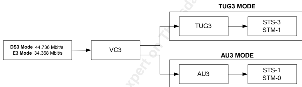
Figure 21 Mapping Structure
