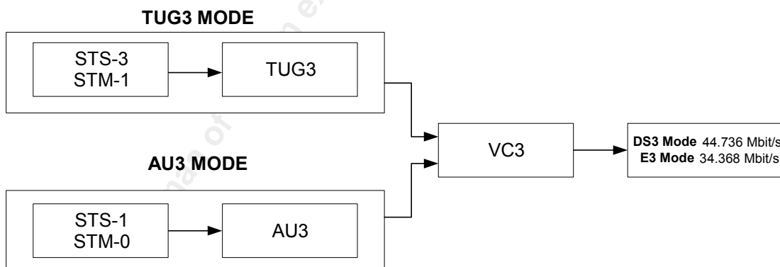
Figure 18 Demapping Structure
