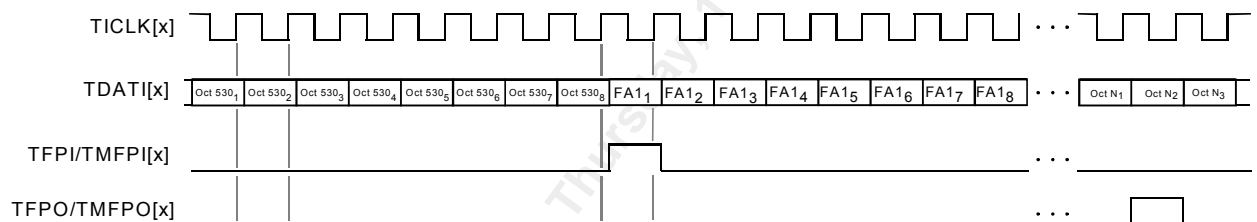
Figure 59 Framer Mode G.832 E3 Transmit Input Stream
