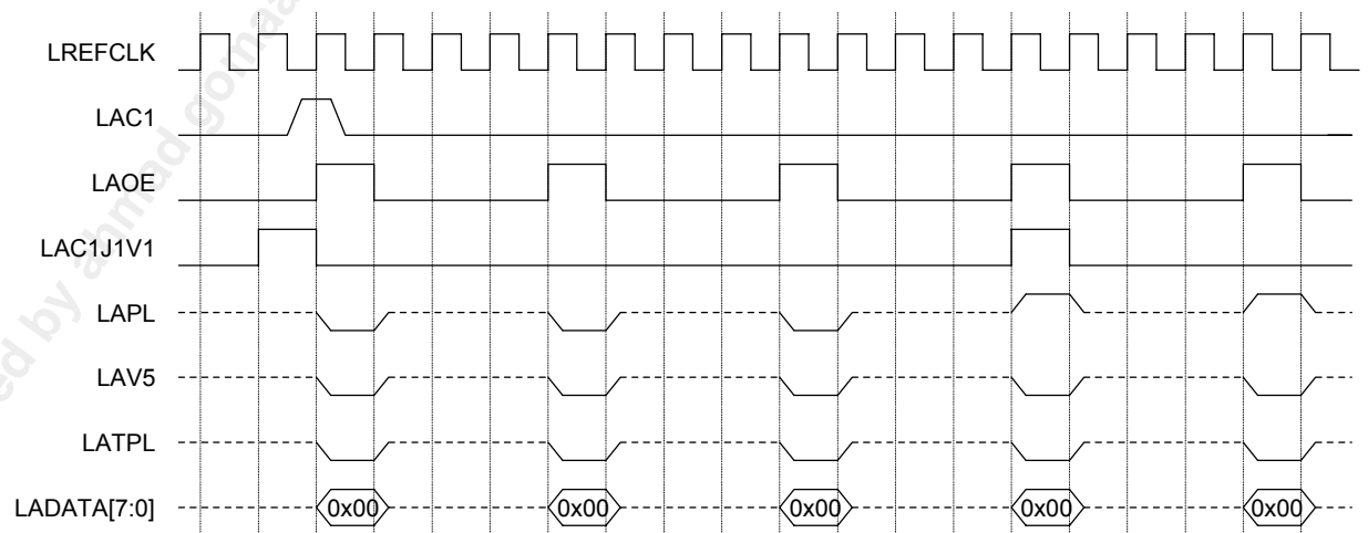
Figure 69 77.76 MHz Telecom ADD Bus Timing
