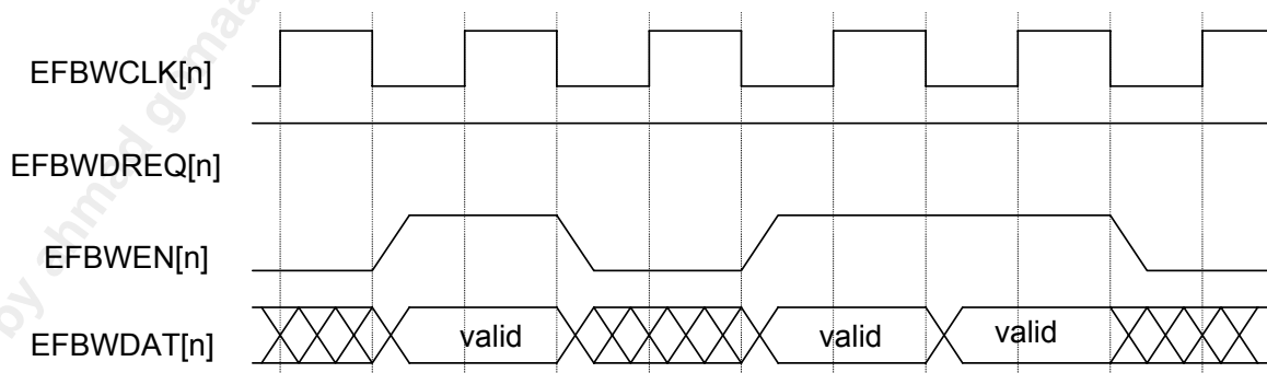
Figure 76 Egress Flexible Bandwidth Port Functional Timing – SBI Slave
