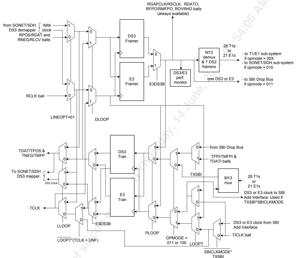
Figure 17 DS3/E3 Configuration Options
