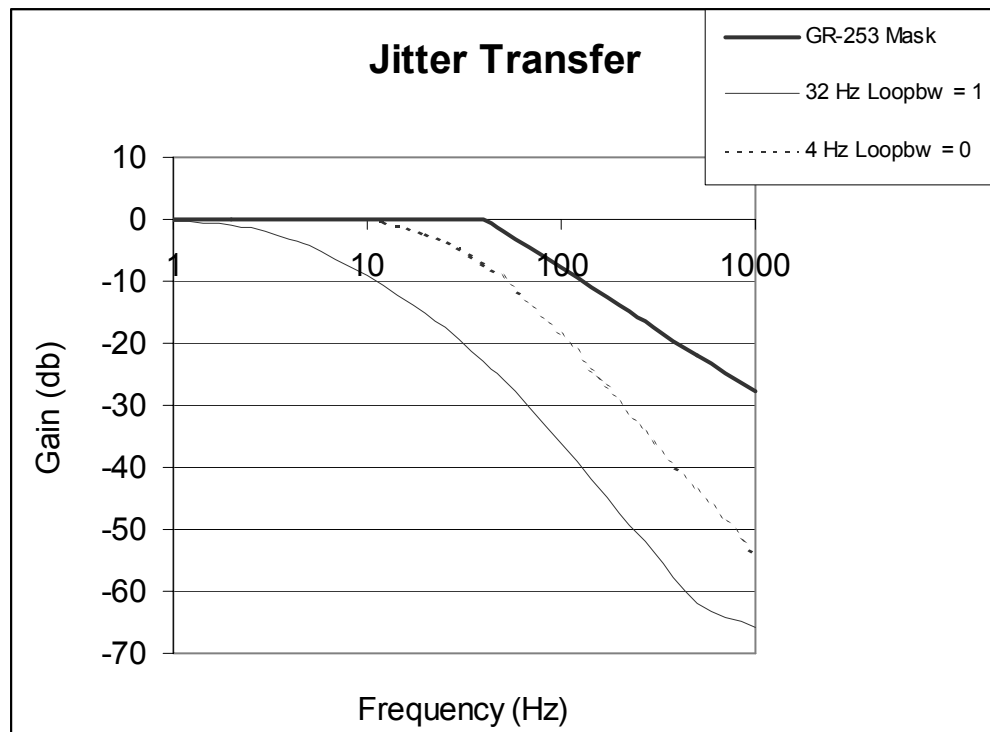
Figure 23 Typical D3E3MA Jitter Transfer
