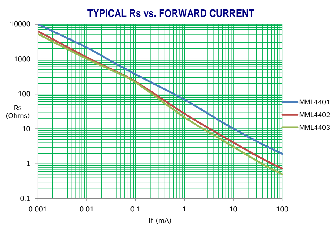
Figure 3 Typical R_s Performance
