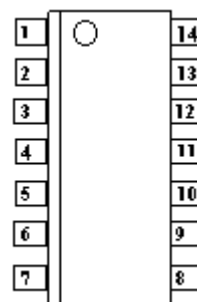
Top Viewing Pin Layout
