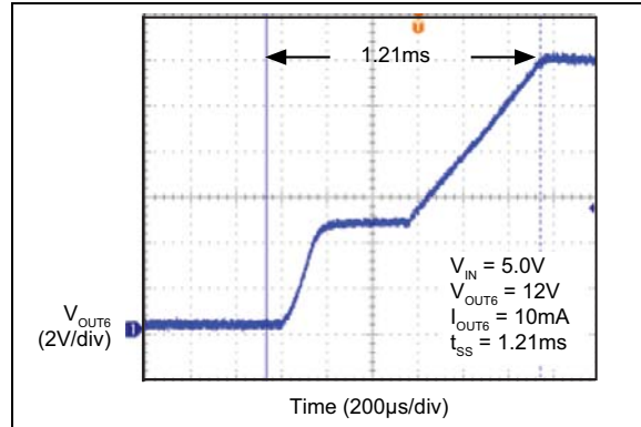
FIGURE 4-6: Boost Soft-Start.
