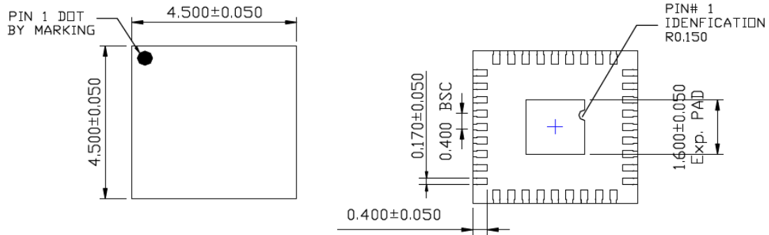
TOP VIEW NOTE: 1, 2, 3
