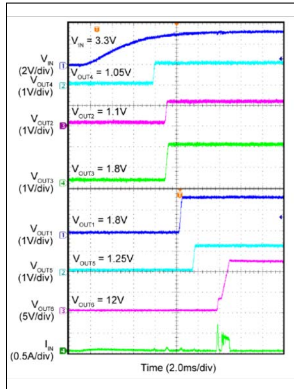
FIGURE 2-45: Input Supply Inrush Current – No Load.
