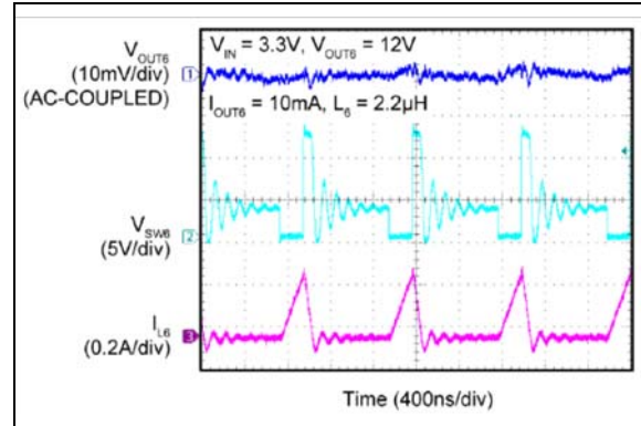
FIGURE 2-44: Boost 6 PFM Switching Waveforms.
