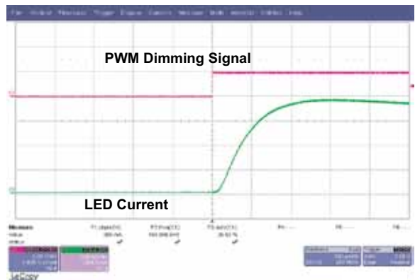
(9b) 300 \mu s - without disconnect FET
