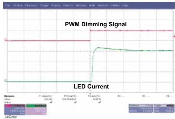
(9a) 5 \mu s - with disconnect FET
