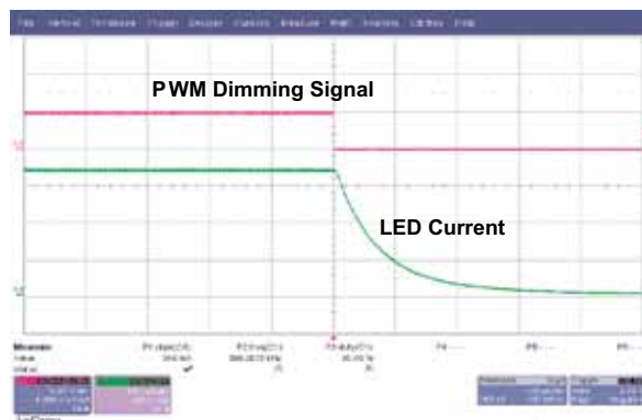
(10b) 300 \mu s - without disconnect FET
