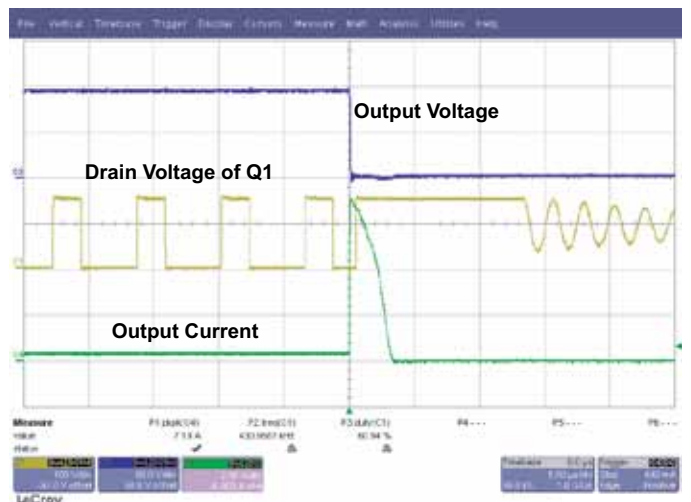
Fig.7 Output Short Circuit Protection
