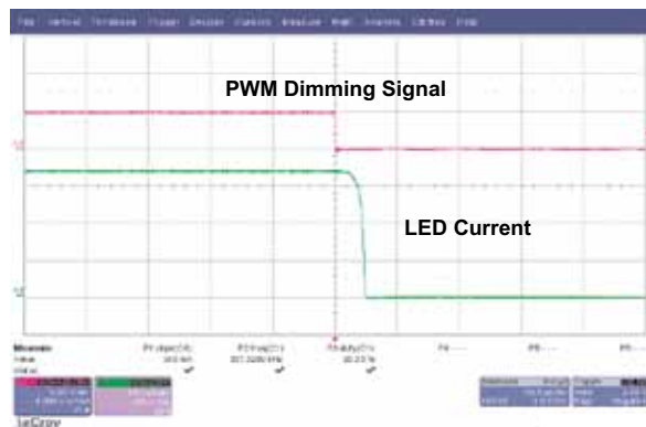
(10a) 5 \mu s - with disconnect FET
