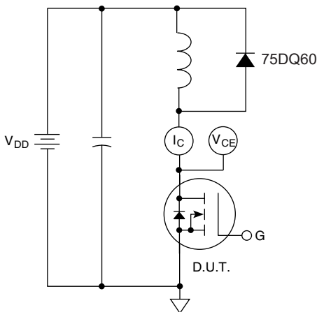
Figure 19, Inductive Switching Test Circuit
