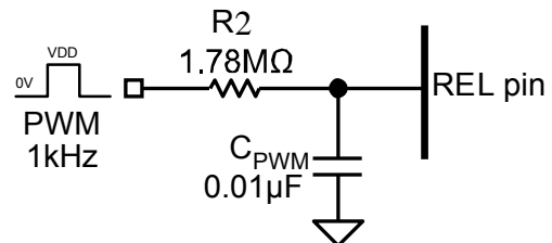
Figure 1. PWM Dimming Circuit
