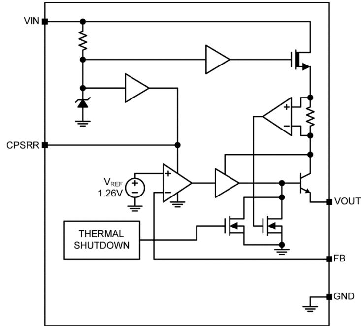
MIC5281 Adjustable Version
