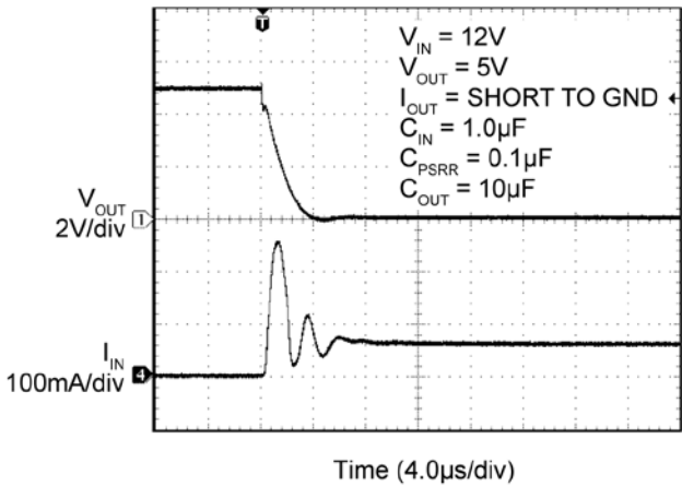
Short-Circuit Response
