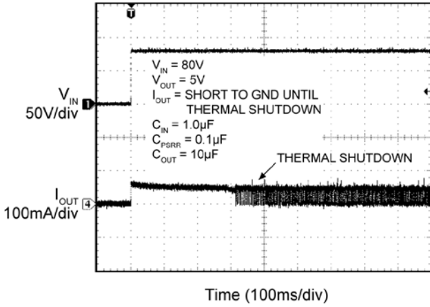
Thermal Shutdown, Short Circuit
